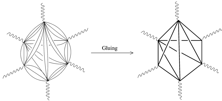
Fig. 1. Gluing up into a skeleton graph.
