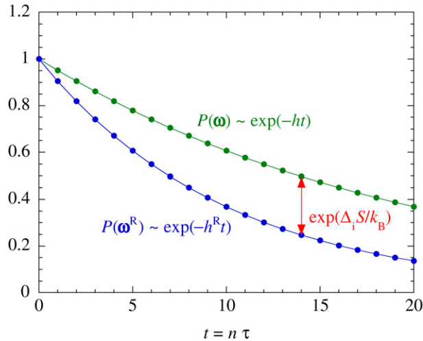
Fig. 1. Diagram showing the probability of a path and the probability of the corresponding time reversal as a function of the number n of time intervals \tau , illustrating the formula (22). \Delta_i S denotes the entropy production during the whole duration n\tau .
