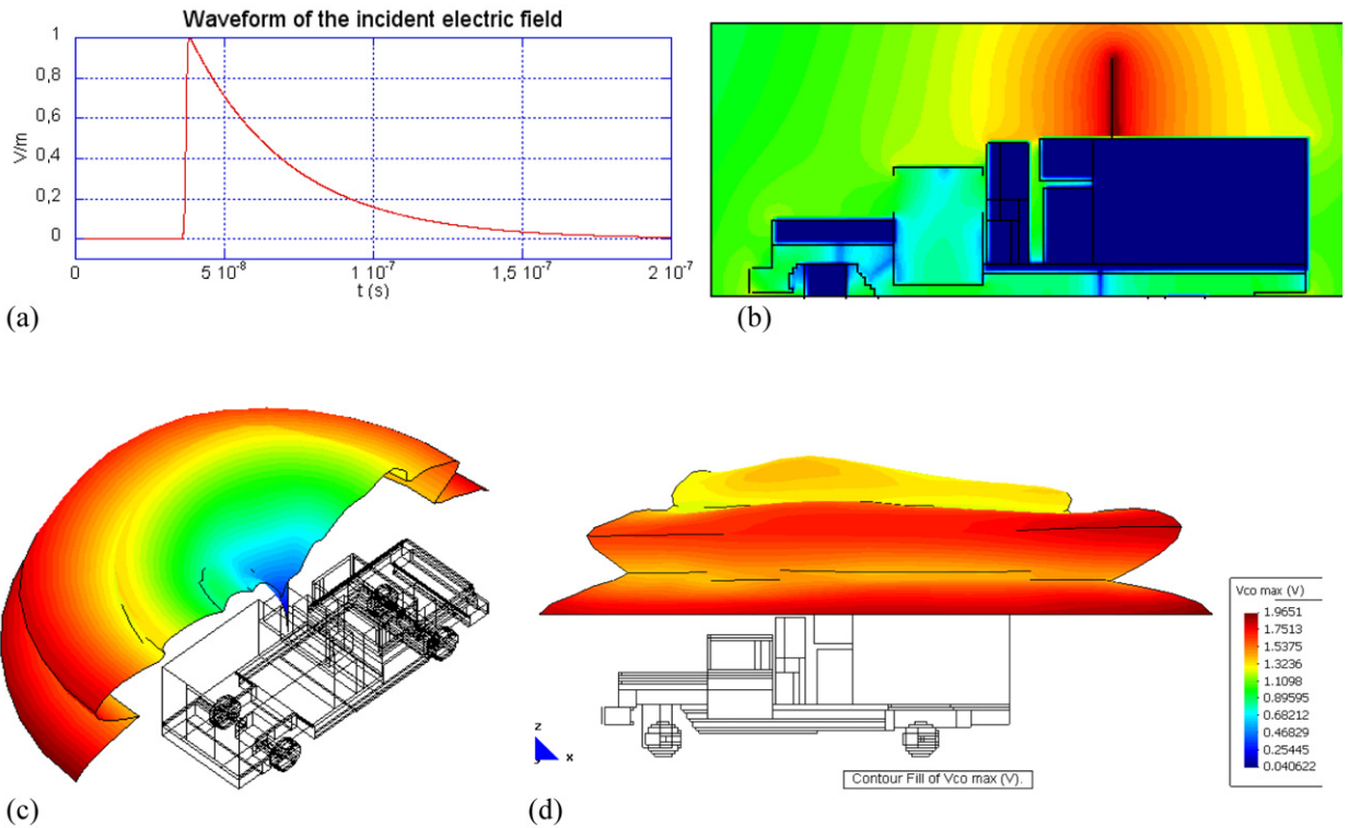
Fig. 2. (a) waveform of the incident field (receiving mode) and of the feeding current (transmitting mode). (b) electric field (log scale) for a given time during the simulation of the monopole fed by a current source. (c) and (d) maximum value of the open circuit voltage induced in the antenna port as a function of the direction of incidence. (c) and (d) are deduced from the simulation shown in (b) with the use of the reciprocity theorem.
