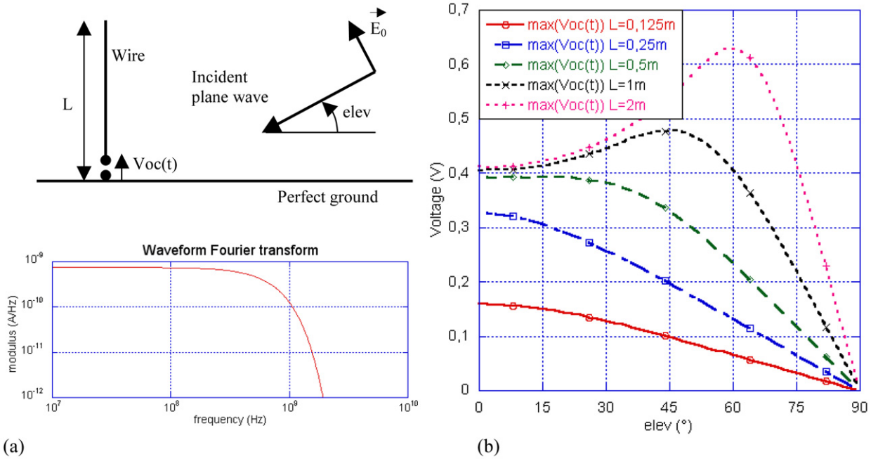
Fig. 1. (a) upper part: monopole antenna in receiving mode; lower part: frequency spectrum of the incident plane wave (receiving mode) and of the feeding current (transmitting mode). (b) maximum value of the open circuit voltage (deduced by reciprocity) as a function of incidence direction, for different monopole lengths.
