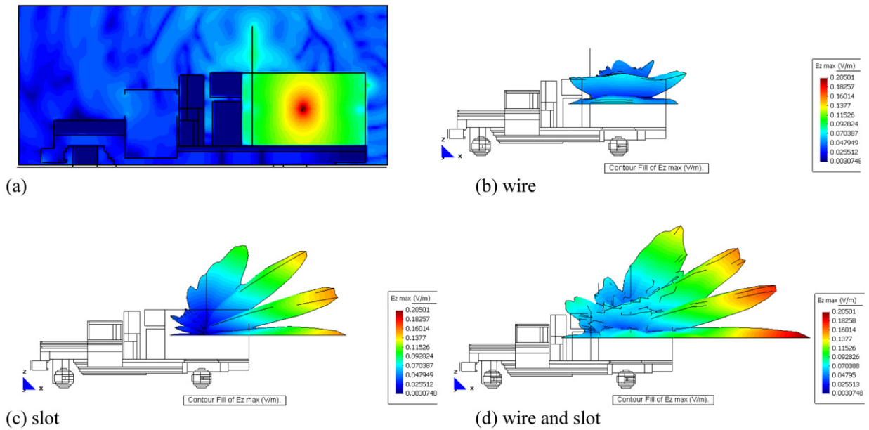
Fig. 3. (a) electric field (log scale) for a given time during the simulation of a small wire fed by a current source. There is a horizontal slot in the rear face. A vertical wire goes through the roof of the truck. (b), (c) and (d) maximum value of the vertical component of the electric field at the small wire location for different directions of incidence. (d) results are deduced by reciprocity from the computation shown in (a). (b) and (c) results are also deduced by reciprocity, but the slot and the wire are respectively absent.
