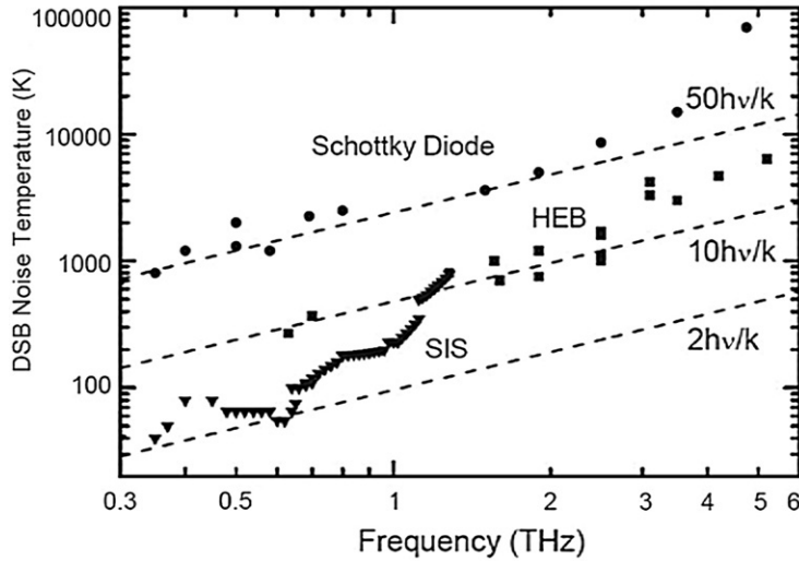
Fig. 9. Double sideband (DSB) noise temperature performance of superconductor–insulator–superconductor (triangles), hot electron bolometer (square), and room-temperature Schottky diode (circle) mixers. The SIS and HEB mixers are cooled between 2 K and 4 K. Also shown are the 2-, 10-, and 50-times quantum noise limit lines for comparison. Reproduced from Chattopadhyay, 2007.
