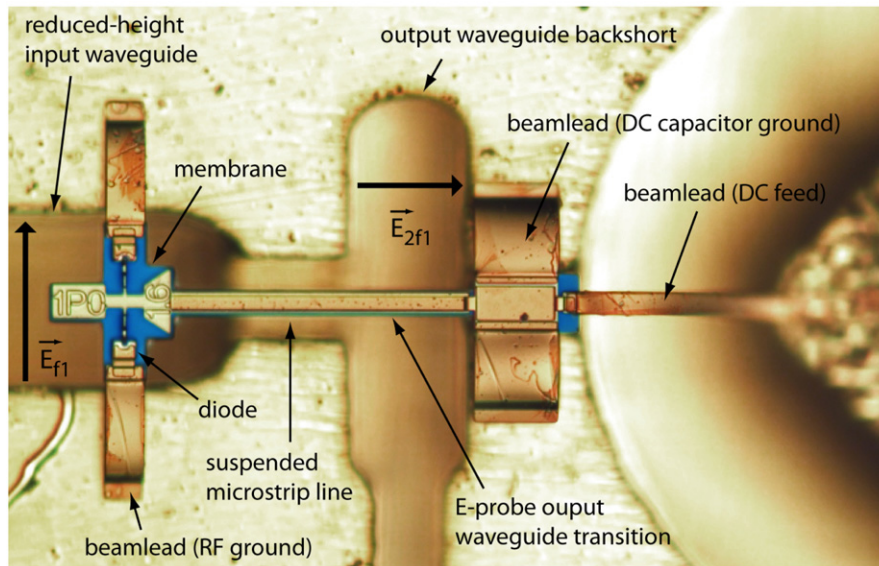
Fig. 6. Photograph of JPL 1500 GHz doubler used to build the 1.5 THz channel of the heterodyne instrument of the Herschel Space Observatory (bottom block with a frame-less 3- \mu\text{m} -thin GaAs membrane device. The chip is approximately 300 \mu\text{m} long.). \vec{E}_{f1} and \vec{E}_{2f1} stand respectively for the electric field at the fundamental frequency f1 and at the output frequency 2 \times f1 .
