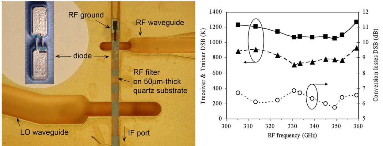
Fig. 11. Photo of a 300–360 GHz sub-harmonic mixer circuit mounted on the lower half of the mechanical block featuring a discrete anti-parallel pair of planar Schottky diodes from the University of Virginia (left) and associated performance (right). The discrete chip from the University of Virginia is 70-μm-wide by 200-μm-long and is mounted onto a 50-μm-thick quartz substrate. The mixer was designed and fabricated at the Observatoire de Paris and shows state-of-the-art performances in this band.
