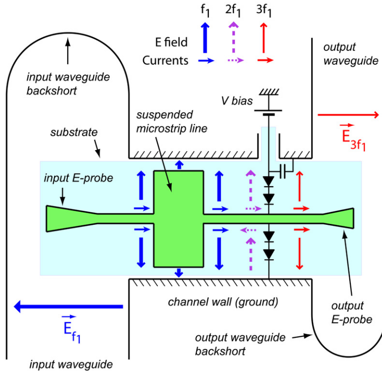
Fig. 4. Block diagram of a 4-anode balanced tripler. The tripler uses a split-block waveguide design. The diodes are connected in series at DC and are in a balanced configuration at RF. The chip is inserted between the input and the output rectangular waveguides in a channel. An E-plane probe located in the input waveguide couples the signal at the fundamental frequency to a suspended microstrip line that can propagate only a quasi-TEM mode. This line has several sections of low and high impedances used to match the diodes at the input and output frequency and to prevent the third harmonic from leaking into the input waveguide. The third harmonic produced by the diodes is coupled to the output waveguide by a second E-plane probe. Additional waveguide sections of different impedances and lengths (not shown) are used for the input and output matching. \vec{E}_{f_1} and \vec{E}_{3f_1} stand respectively for the electric field at the fundamental frequency f_1 and at the output frequency 3 \times f_1 . The electric fields and the current lines are represented for the fundamental frequency f_1 (thick plain lines), the idler frequency 2 \times f_1 (dashed lines) and the output frequency 3 \times f_1 (light plain lines).
