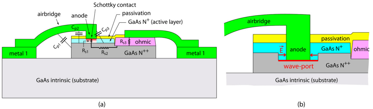
Fig. 2. Left view (a): schematic of a planar Schottky diode. C_p stands for parasitic capacitance and R_s for series resistance. Note that R_{s3} is the series resistance introduced by the ohmic contact at DC. At RF the currents flow principally on the surface of the conductors and R_{s3} has a different value. Right view (b): wave port at the location of the Schottky contact as implemented in the electromagnetic field solver. The N^+ layer is modeled as an intrinsic GaAs layer while the N^{++} layer is modeled as a non-perfectly conductive metallic layer. These approximations are made to implement the port that can be seen as an electromagnetic-field probe/emitter.
