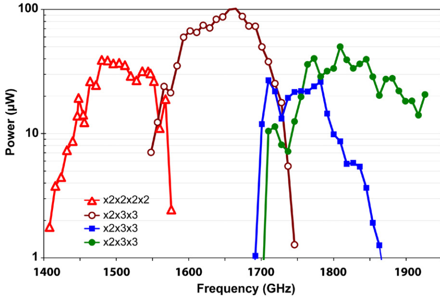
Fig. 5. Performance of 1.4–1.6 THz (open triangles), 1.6–1.7 THz (open circles) and 1.7–1.9 THz (squares and filled circles) local oscillator chains developed for the heterodyne instrument of the Herschel Space Observatory at 120 K.
