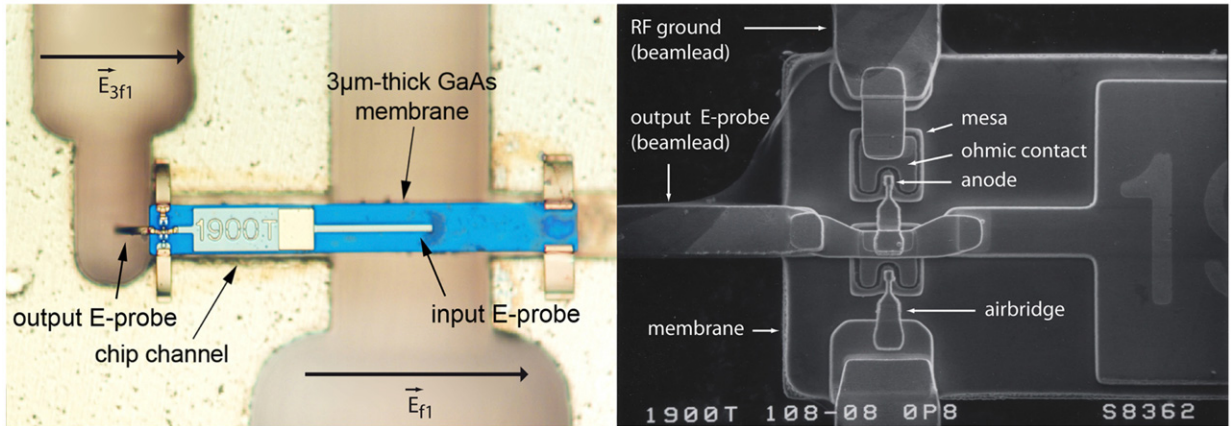
Fig. 7. Top view: photograph of JPL 1.9 THz tripler used to build the 1.7–1.9 THz channel of the heterodyne instrument of the Herschel Space Observatory (bottom block with a frame-less 3- \mu\text{m} -thin GaAs membrane device). \vec{E}_{f_1} and \vec{E}_{3f_1} stand respectively for the electric field at the fundamental frequency f_1 and at the output frequency 3 \times f_1 . The chip is approximately 290 \mu\text{m} long. Bottom view: SEM picture of a 1.9 THz tripler chip.
