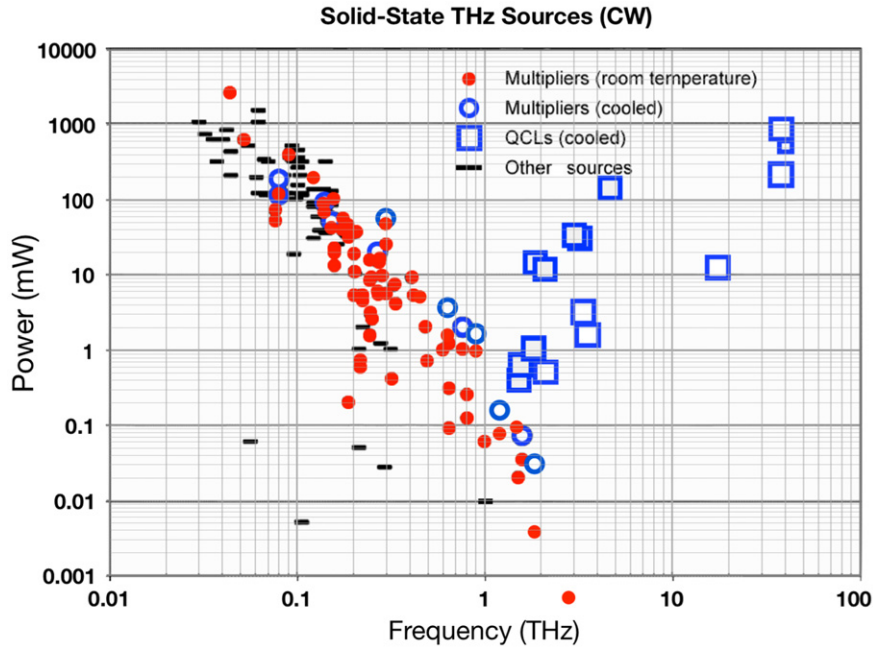
Fig. 1. Terahertz gap with respect to source technology. Quantum cascade lasers ( \square ) are progressing downward from higher frequencies, while electronic technology is progressing upward. Frequency multipliers ( \circ ) dominate other electronic devices ( - ) above about 150 GHz. Cryogenic results are shown as hollow symbols. Adapted from T. Crowe et al., IEEE J. Solid-State Circuits 40 (10) (October 2005) 2104–2110. New data added by the author, December 2009.
