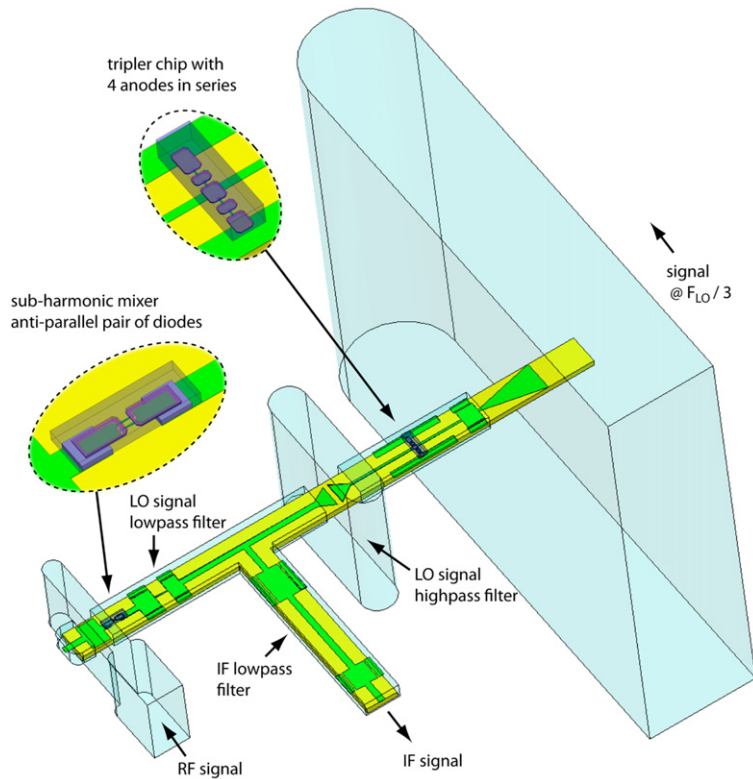
Fig. 13. 3D view of the circuit as modeled in the 3D-electromagnetic field solver. In this model, the RF waveguide, the IF channel and the LO input waveguide are all coming from the same side since it does not have any impact on the simulations. For the fabrication of the circuit, however, one of the waveguides or the IF channel has to be rotated by 180° or bent at 90°.
