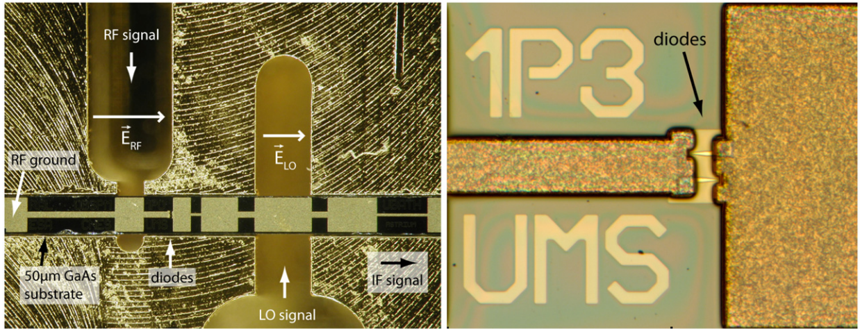
Fig. 12. Photo of a 183 GHz sub-harmonic mixer circuit mounted on the lower half of the mechanical block featuring a 4-mm-long MMIC device on a 50-μm-thick GaAs substrate from United Monolithic Semiconductors (left). For the final assembly, the device is actually flipped at 180° and connected to the block using a silver-epoxy conductive glue (so only the back of the device can be seen). The right view shows a closeup of the diode region. This mixer was designed at the Observatoire de Paris.
