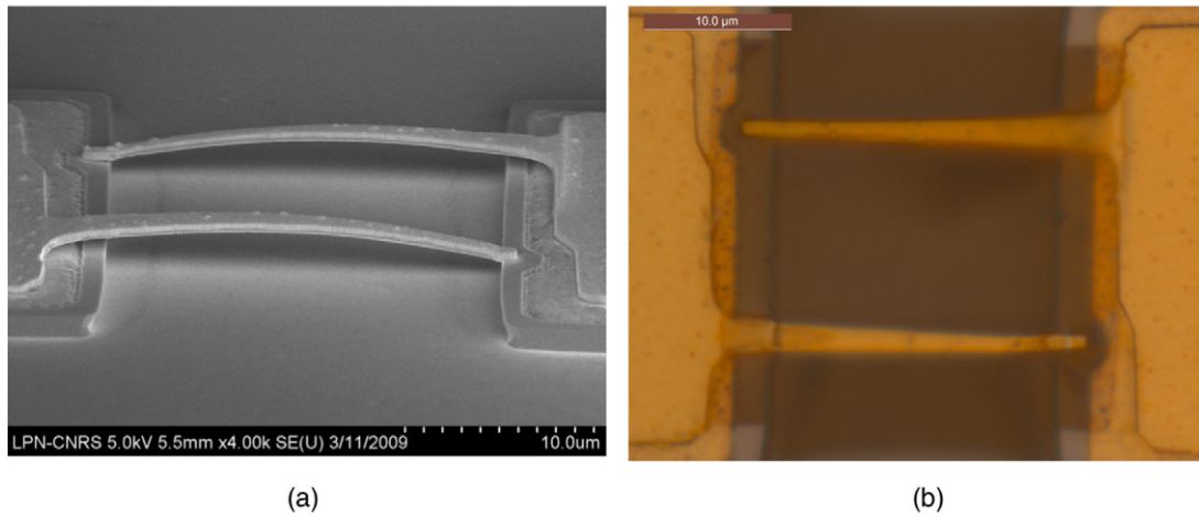
Fig. 14. SEM picture of an antiparallel pair of Schottky diodes fabricated at LPN for a 300–360 GHz sub-harmonic mixer (a) and optical picture of a similar antiparallel pair of diodes (b).
