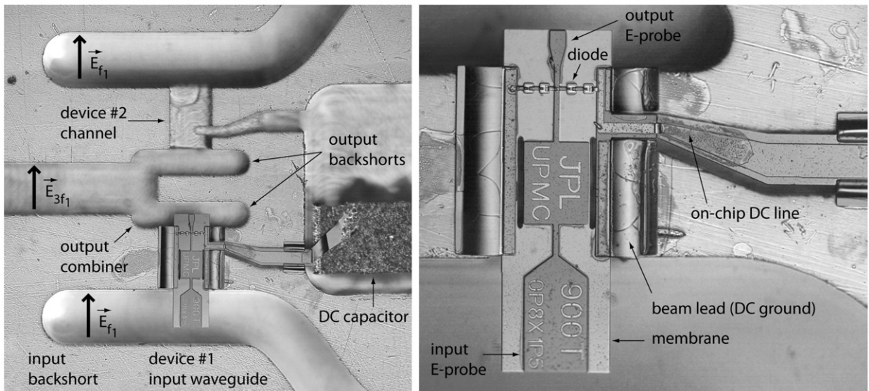
Fig. 8. Photograph of the bottom block of a 900 GHz dual-chip frequency tripler with one membrane device mounted. The second device is mounted in the top block which is exactly symmetrical. The chip is approximately 325 \mu\text{m} long and 100 \mu\text{m} wide.
