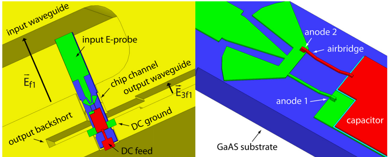
Fig. 3. Schematics of a submillimeter wave frequency tripler using an anti-parallel pair of diodes. Left: bottom block with the integrated device. Right: detail of the anode area. \vec{E}_{f1} and \vec{E}_{3f1} stand respectively for the electric field at the fundamental frequency f1 and at the output frequency 3 \times f1 .
