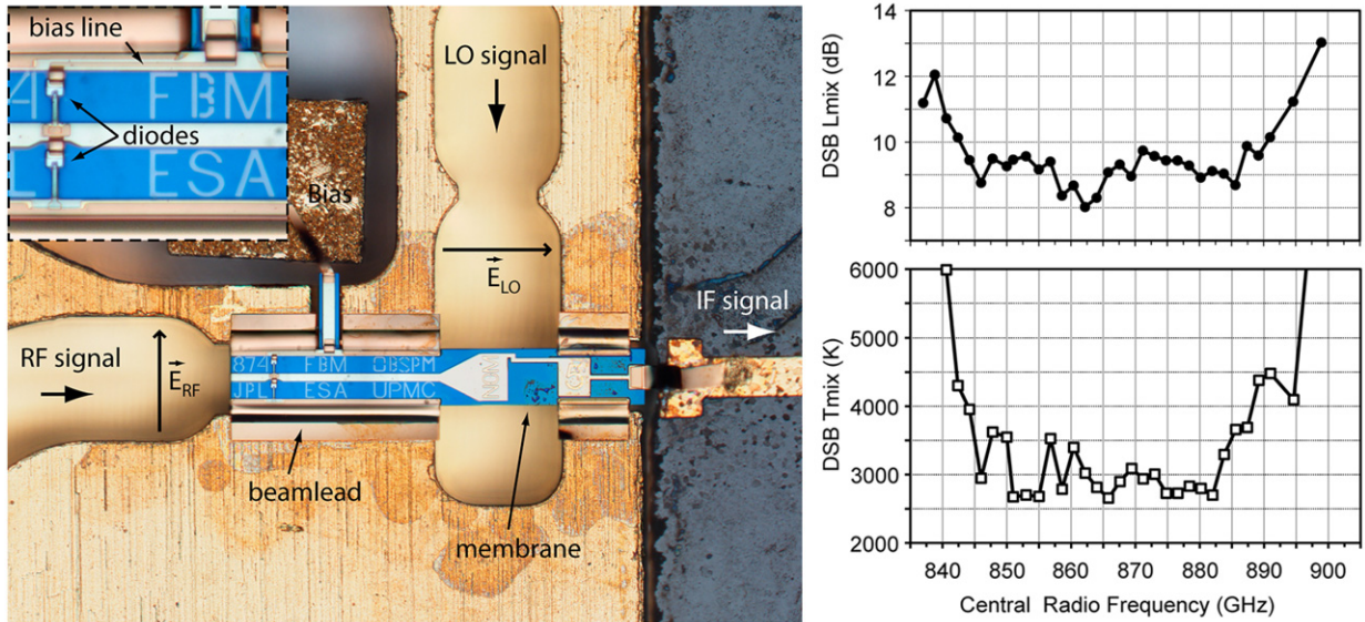
Fig. 10. Photograph of a 840–900 GHz fundamental balanced mixer circuit mounted on the lower half of the mechanical block featuring MMIC Schottky diodes device from JPL (left) and associated performance (right). The top-right curve (plain circles) shows the mixer DSB conversion losses L_{mix} for a radio frequency ranging from 840 GHz to 900 GHz. The bottom-right curve (open squares) shows the corresponding DSB mixer equivalent noise temperature T_{mix} . \vec{E}_{RF} , \vec{E}_{LO} stand respectively for the electric field at RF and LO frequency. The chip is approximately 530 \mu\text{m} long.
