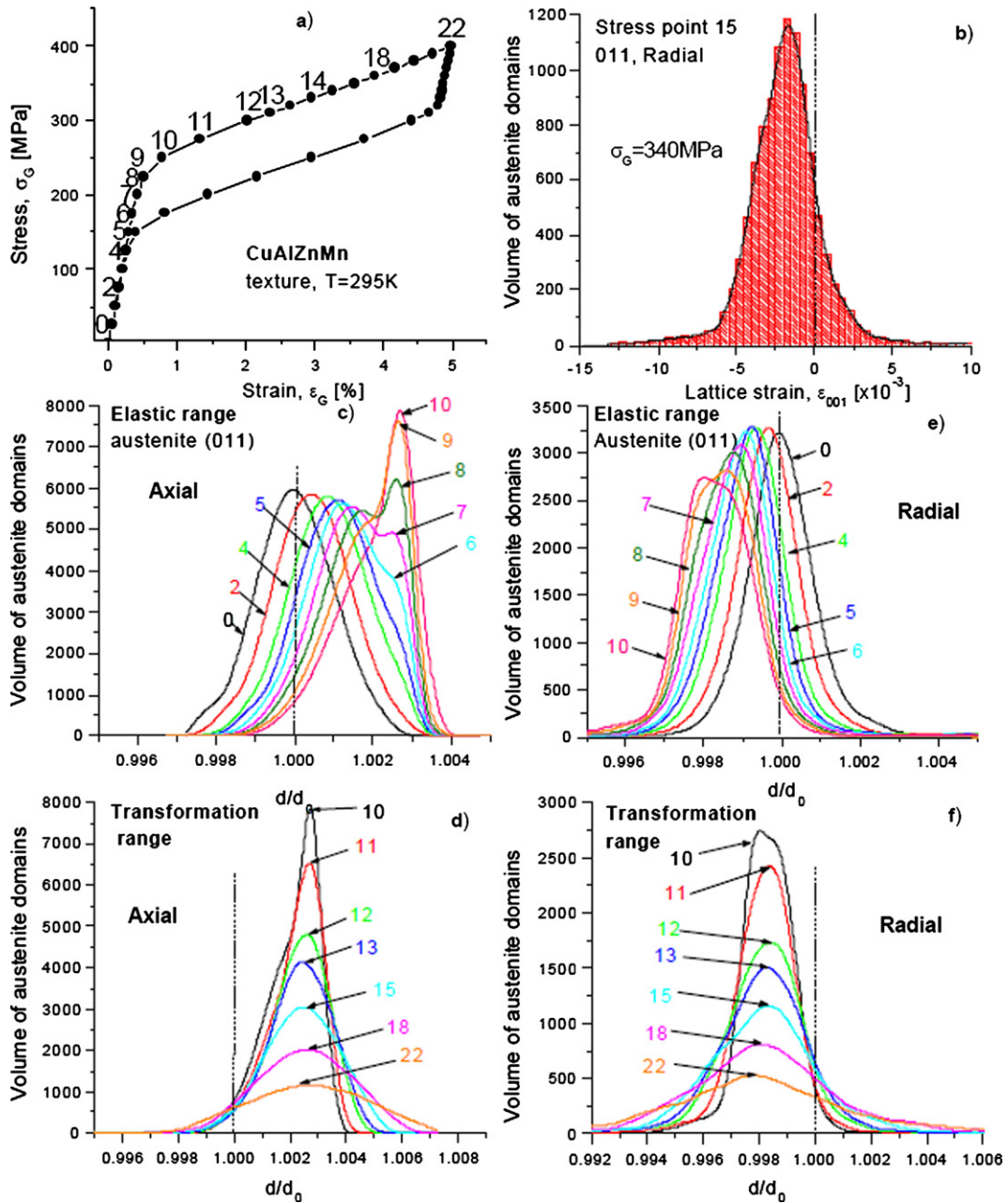
Fig. 4. CuAlZnMn polycrystal in tension at T = 295 K. Simulated distributions of the d_{011} -lattice spacing in stress points 0 to 22 during forward loading (a), in axial configuration (c,d), and in radial configuration (e,f). The profiles in (c–f) were obtained as envelope curves of the histograms informing the fraction of {011} oriented domains with particular lattice strain (as the one in (b) for stress point 15 and radial configuration) [8].
