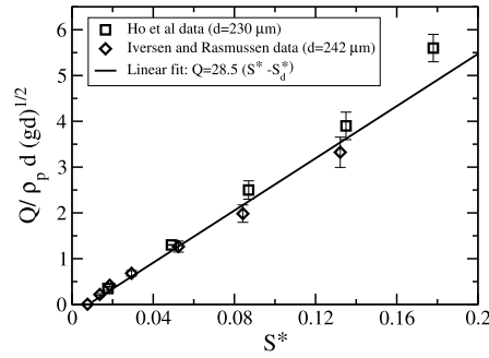
Fig. 7. Mass flow rate versus the Shields parameters obtained from wind-tunnel experiments with sand grains of mean diameter d = 230 \mu\text{m} [26] and d = 242 \mu\text{m} [11], respectively.
