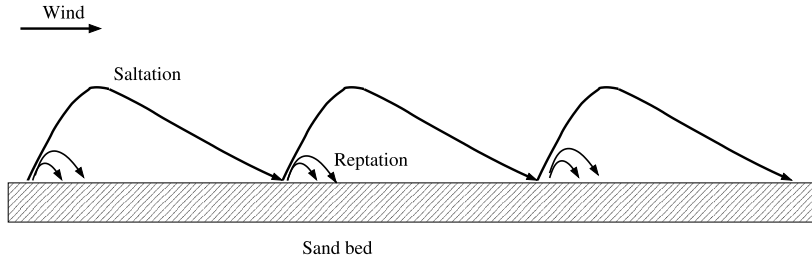
Fig. 1. Schematic of the different modes of Aeolian sand transport: (i) saltation mode and (ii) reptation mode.
