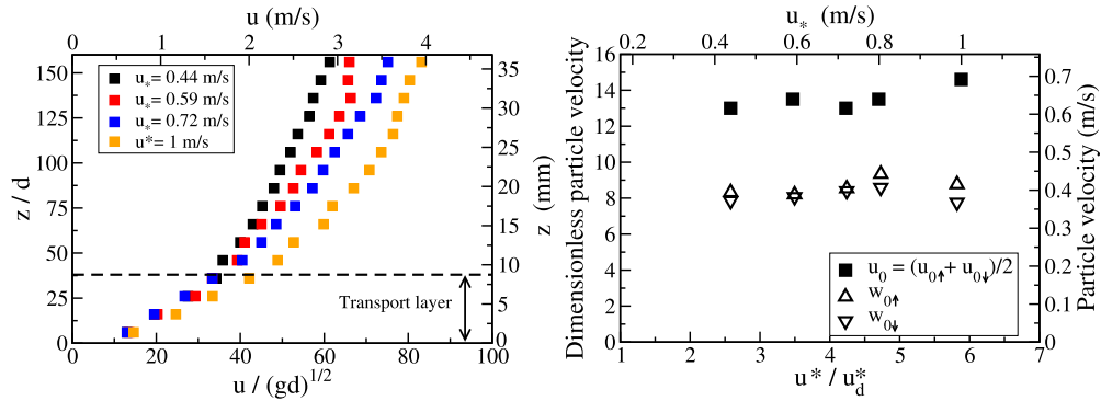
Fig. 4. (Color online.) (a) Average particle velocity profiles obtained with natural sand of median diameter d = 230 \mu\text{m} for various wind strengths ( u^* = 0.44, 0.59, 0.72, 1 \text{ m/s} ) [10]; (b) Average horizontal slip velocity u_0 and average vertical velocity of upward and downward particles close to the bed surface ( w_{0\uparrow} and w_{0\downarrow} ) versus the friction velocity [10].
