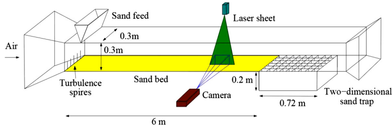
Fig. 3. (Color online.) Wind tunnel used by Ho et al. [26] for characterizing the saltation transport using Particle Image Velocimetry and sand trap system.
