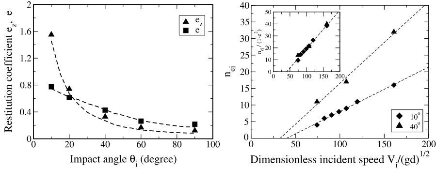
Fig. 10. Experimental data from model collision experiments with 6-mm PVC beads [38]: (a) Variation of the average restitution coefficient e_z and e as a function of the impact angle \theta_i for a fixed impact velocity \xi_i = 106\sqrt{gd} = 26 m/s. The dotted lines stand for best fits of the form: A_z/\sin\theta_i - B_z for e_z (with A_z = 0.30 and B_z = 0.15 ), and A - B \sin\theta_i for e (with A = 0.87 and B = 0.72 ). (b) Mean number of ejected beads versus the impact speed for two different impact angles, \theta_i = 10^\circ ( \blacklozenge ) and 40^\circ ( \blacktriangle ).
