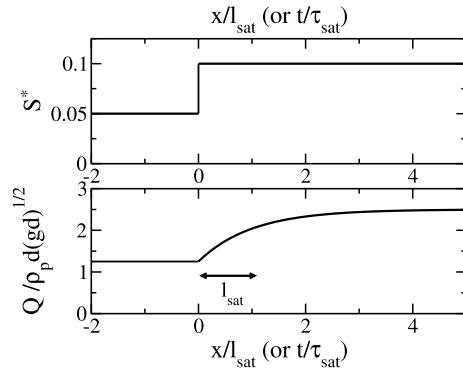
Fig. 11. Spatial (or temporal) variation of the mass flow rate Q over a sand bed following an increase of the wind speed: the mass flow rate relaxes to its new saturation value within a saturation length l_{\text{sat}} .
