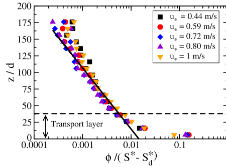
Fig. 6. (Color online.) (a) Particle volume fraction profiles rescaled by (S^* - S_d^*) obtained with natural sand of median diameter d = 230 \mu\text{m} for various wind strengths ( u_* = 0.44, 0.59, 0.72, 0.80, 1 \text{ m/s} ). (Wind-tunnel experiments by Ho [10].)
