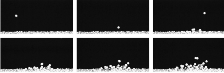
Fig. 9. Successive Snapshots of a collision of a 6-mm PVC bead onto a granular packing of like particles [38]. The impact velocity and angle are, respectively, \xi_i = 74\sqrt{gd} = 18 m/s and \theta_i = 40^\circ and the collision. The time step between two successive images is 4 ms.
