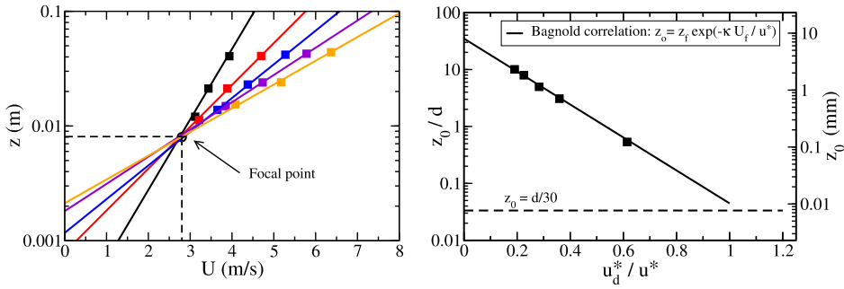
Fig. 2. (Color online.) (a) Air velocity profiles obtained with natural sand of median diameter d = 230 \mu\text{m} for various wind strengths ( u^* = 0.28, 0.47, 0.60, 0.75, 0.89 \text{ m/s} ) [10]; (b) Aerodynamic roughness length z_0 as a function of u_d^*/u^* [10].
