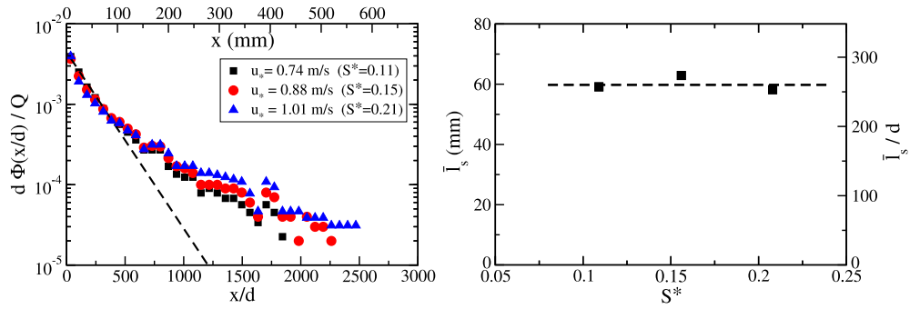
Fig. 8. (Color online.) (a) Vertical mass flux distribution d\Phi(x)/Q for various Shields parameters (experimental data by Ho et al. [32] with 230 \mu m sand). Note that we have normalized the distribution \Phi(x) by the mass flow rate Q such that \int_0^\infty dx\Phi(x)/Q = 1 . The dash line represents the best fit to the data obtained with an exponential law. (b) Dimensionless saltation length \bar{l}_s/d versus the Shields (experimental data by Ho et al. [32] with 230- \mu m sand).
