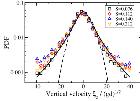
Fig. 5. (Color online.) Vertical velocity distribution p(\xi_z) of saltating particles located close to the bed surface within the transport layer (at z = 10d ) for various wind strengths obtained from wind-tunnel experiments [27]. Fitted distributions: (dashed line) Gaussian law with variance s^2 = 53gd and (solid line) lognormal law.
