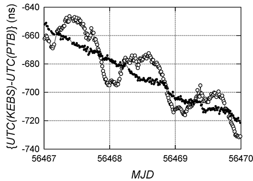
Fig. 1. GPS CV time comparisons between Kenia Bureau of Standards and PTB; open symbols: L1C single frequency data, full symbols: dual frequency L3P data obtained from the same receiver; acronyms are explained in the text below.
