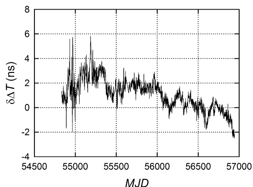
Fig. 8. Long-term assessment of time comparison UTC(OP)–UTC(PTB), double-difference between GPS P3 and TWSTFT data (daily mean values), data by courtesy of Pierre Uhrich, SYRTE, data span 2009 until October 2014.
