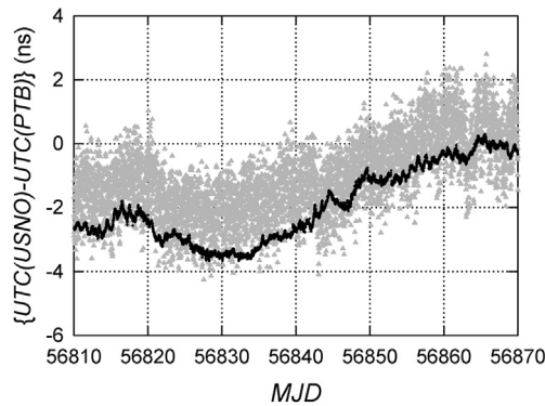
Fig. 2. Time comparison UTC(USNO)–UTC(PTB) via GPS P3 (grey symbols) and GPS PPP (black symbols) during the months June and July 2014 (16-min averages). Source of data: BIPM ftp server (see text); the small but apparent offset between the two data sets is likely caused by the fact that the USNO data come from two different GPS receivers.
