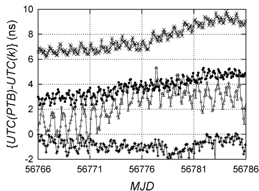
Fig. 6. TWSTFT providing UTC(PTB) - UTC(k) during twenty days in April 2014, k = \text{IT} (INRIM), (symbol \Delta ), OP (SYRTE) (symbol \bullet ), NIST (symbol \times ) and USNO (symbol + ).
