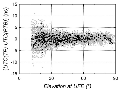
Fig. 3. CV time comparison UTC(TP)–UTC(PTB) via GPS (grey symbols) and Galileo (black symbols) during five days in April 2014 (5-min averages), results of individual satellite observations. The daily mean time scale difference was subtracted from the data. TP stands for Tempus Pragensis, UTC(TP) is realized at UFE (Prague). The horizontal axis denotes the elevation of the satellite in common view above Prague.
