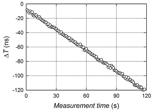
Fig. 4. Reception of TWSTFT signals transmitted from SYRTE (Observatoire de Paris) at PTB on 2014-05-08 between 02:19:00 and 02:20:59 UTC (120 points). \Delta T represents the time difference recorded minus 0.26458 s.
