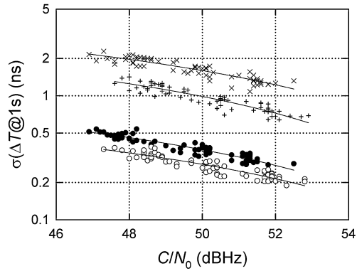
Fig. 7. Scatter of 1-s ranging measurement results, \sigma(\Delta T@1s) , recorded at PTB using different PN chip rates: ( \times ) 0.5 MChip/s, ( + ) 1 MChip/s, ( \bullet ) 2.5 MChip/s, ( \circ ) 5 MChip/s. The use of 2.5 MChip/s was common at the time when the data were taken, but was later given up for cost reasons.
