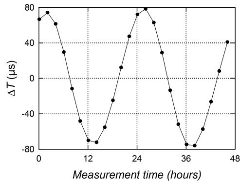
Fig. 5. Example for ranging results: Reception of TWSTFT signals transmitted from PTB at PTB on 2014-05-07 and 2014-05-08, 12 points per day; each point represents the mean over the 120 data points collected between 00:07:00 and 00:08:59. \Delta T represents the time difference recorded minus 0.2667 s, note the scale is \mu\text{s} (not ns as in Fig. 4).
