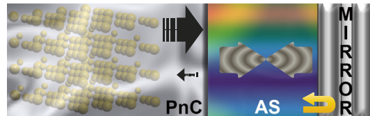
Fig. 5. Harvesting vibrations via a 3D PnC, an absorbing slab (AS) and an acoustic mirror.
