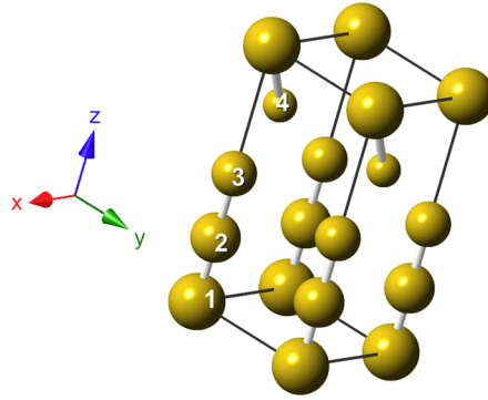
Fig. 1. Unit cell of a monoclinic PnC with a four-point basis. The crystal is viewed as a succession of four nonprimitive planes of spheres parallel to the (001) surface at positions (0, 0, 0) , (0, 0, a/2) , (0, 0, a) , and (0.3a, 0, 3a/2) . The radius of Au spheres for each plane is S_1 = 0.30a , S_2 = 0.25a , S_3 = 0.20a , and S_4 = 0.15a , respectively. The four-point basis of the Bravais lattice is designated by the thick grey links.
