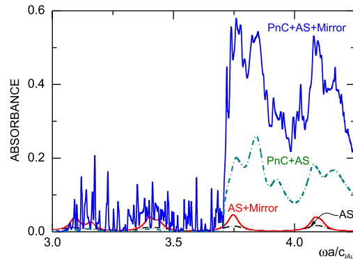
Fig. 6. Absorbance for a compressional elastic wave incident at \mathbf{k}_{\parallel} = (\pi/4, 0)/a on different types of slab sequences. AS: absorbing slab [ c_{IAS} = 2c_{le}(1 - i10^{-3}) ] of thickness d = 10a . AS + Mirror: absorbing slab on top of a perfect mirror. PnC + AS: 16-layer PnC slab on top of the absorbing slab. PnC + AS + Mirror: 16-layer PnC slab on top of the absorbing slab and perfect mirror.
