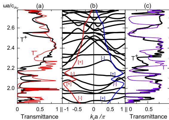
Fig. 2. Asymmetric transmittance for a compressional elastic wave (a) and a p-polarized shear (c) for oblique incidence at \mathbf{k}_{\parallel} = (\pi/4, 0)/a on a finite slab of the PnC (see Fig. 1) consisting of 8 unit layers. T^+ and T^- correspond to the transmittance associated with wave incidence from the left and right (001) faces of the slab, respectively. (b) Frequency band structure of the infinitely periodic PnC for \mathbf{k}_{\parallel} = (\pi/4, 0)/a .
