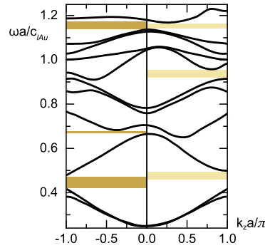
Fig. 3. Frequency band structure of the infinitely periodic PnC at a different direction from Fig. 2, defined by \mathbf{k}_{\parallel} = (\pi/8, \pi/8)/a . Asymmetry is manifested through the formation of unidirectional frequency gaps.
