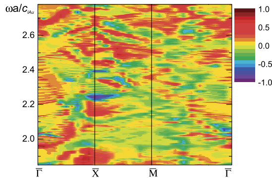
Fig. 4. Transmission difference, recorded as \Delta T = T^+ - T^- , for a p -polarized shear wave incident from the left ( T^+ ) and right ( T^- ) faces of an 8-layer slab of the PnC of Fig. 1, projected on the SBZ of the (001) surface along its symmetry points.
