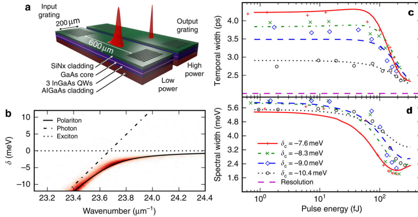
Fig. 6. (a) Schematic diagram of waveguide (the same waveguide is shown with pulses under low-power and high-power excitation conditions). (b) Angle-resolved photoluminescence spectrum showing emission from the lower polariton branch in red. The fitted polariton dispersion (solid line) is shown with the uncoupled exciton and photon modes, which would exist for zero light matter coupling (dotted and dashed lines). The horizontal and vertical axes are respectively the wavenumber of the guided mode and the detuning \delta between polariton and exciton energies. (c) Experimental (symbols) and numerically simulated (line) pulse temporal duration versus pulse energy inside the waveguide for a number of detunings \delta_c of the central pulse frequency from the exciton. (d) Experimental (symbols) and numerically simulated (lines) pulse spectral width versus pulse energy for the same detunings. Adapted from [27].
