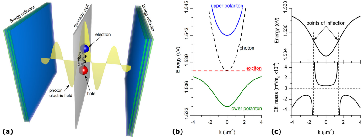
Fig. 1. (a) Schematic of a microcavity with quantum well positioned at an antinode of a photon mode. (b) Simulated polariton dispersion of a typical GaAs microcavity. Black dashed line is dispersion of uncoupled photons, red dashed – uncoupled exciton, blue solid – upper polariton branch, and green solid – lower polariton branch. (c) Lower polariton branch, upper panel, and corresponding effective mass, lower panel, as a ratio to free electron mass ( m_0 ) show two points of inflection which divide regions of positive and negative effective masses of polaritons.
