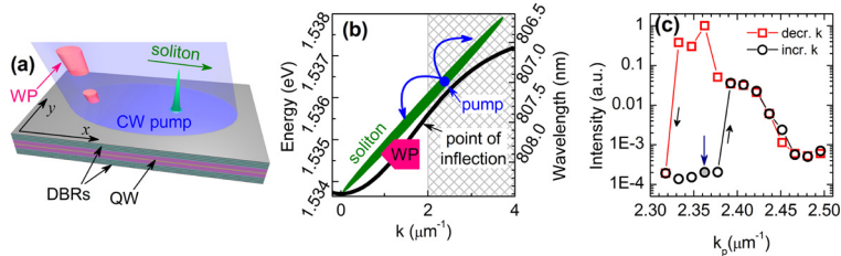
Fig. 7. (a) Schematic diagram of experiment. A large area of the sample is quasi-resonantly illuminated with a continuous wave (CW) pump. A picosecond writing pulse (WP) (red) triggers the soliton pattern formation. (b) Polariton dispersion (solid black curve) of the lower polariton branch (LPB). The schematic location of the pump and WP in energy–momentum space are shown; in the experiment the shaded area above k > 2 \mu\text{m}^{-1} is blocked in the detection path to avoid saturation of the detectors by the reflected pump and WP beams. (c) Bistable polariton density as a function of pump momentum. Arrow indicates the state of the system created by the pump before incidence of the writing pulse. Adapted from [25].
