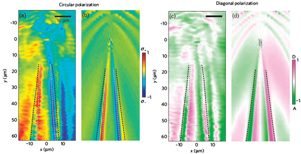
Fig. 3. (a), (c) The measured degree of circular and diagonal polarisations, respectively; (b), (d) The calculated patterns from the solution to the nonlinear spin-dependent Schrödinger equation. The dashed lines show the trajectory of the inner (grey) and outer (black) half-solitons. The trajectories of the half-solitons appear as extremes of circular polarization, and as domain walls in diagonal polarization. The grey arrows in (b) indicate the direction of acceleration of the half-solitons induced by the effective magnetic field.
