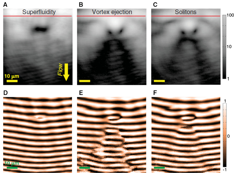
Fig. 2. (A to C) Real-space images of the polariton gas flowing downward at different excitation densities in the presence of a double defect (total width: 15 \mu\text{m} ). The gas is injected above the red line. At high density (A) (117 mW), the fluid is subsonic ( v_{\text{flow}} = 0.25c_s ) and flows in a superfluid fashion around the defect. At lower densities (B) (36 mW; v_{\text{flow}} = 0.4c_s ), a turbulent pattern appears in the wake of the defect, eventually giving rise to the formation of two oblique dark solitons (C) (27 mW; v_{\text{flow}} = 0.6c_s ). (D to F) Interferograms corresponding to (A) and (C), respectively. From [24]. Reprinted with permission from AAAS.
