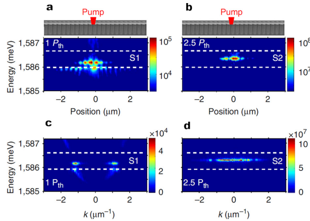
Fig. 4. A modulated wire is excited with a 2 \mu\text{m} CW laser spot centred on a maximum of the periodic potential (narrow region of the wire). Total emission intensity measured from a single modulated wire as a function of the excitation power. (a, b) Spectrally and spatially resolved emission for two excitation powers (in logarithmic colour scale). (c, d) Spectrally resolved far-field emission measured on the same wire for the same excitation powers (in linear colour scale); the first mini-gap induced by the periodicity is indicated with dashed lines.
