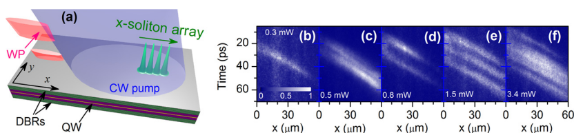
Fig. 9. (a) Experimental setup is similar to that shown in Fig. 7(a), but with a significantly elongated WP beam. (b–f) Emission intensities of a single soliton (b) and x -soliton arrays (c–f) for different WP powers recorded versus time and position x ; t \approx 0 is the WP arrival time within an error of 5 ps. The pump beam is centred around x = 30 \mu\text{m} .
