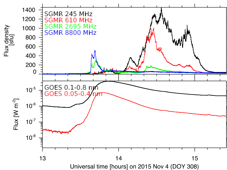
Fig. 2. Time history of whole-Sun X-ray and radio emissions during a solar flare/CME event. Bottom: soft X-rays in two wavelength ranges (GOES satellites, NOAA). Top: radio waves at selected frequencies (RSTN, US Air Force). From Marqué et al. (2017, submitted to Journal of Space Weather and Space Climate ).
