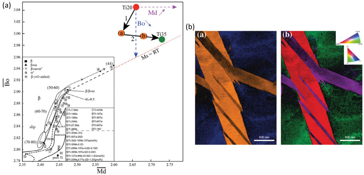
Fig. 5. (a) Bo-Md map used for conventional Ti-based alloys (bottom left) extrapolated to concentrated Ti alloys (top right) [89]. The dashed line corresponds to the formation of martensite ( M_s ) from the bcc \beta phase. Starting from the equimolar HfNbTaTiZr composition, the coupled reduction of Ta and Nb contents and the increase of Hf, Nb and Ti ones lead to the definition of a non-equiatomic HfNbTaTiZr composition close to the martensite appearance zone; (b) Presence of stress induced \alpha' (hcp) martensite in the initial \beta (bcc) phase after deformation. Phase mapping (left; bcc: blue; hexagonal: orange) and orientation mapping (right) (from [86]).
