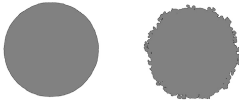
Fig. 7. Example of shapes obtained for the model M_1 . (Left) Constant emission rate and \ell = 10 . (Right) Emission rate proportional to the perimeter (Eq. (13)), and \ell = 2 . Figures taken from [37].
