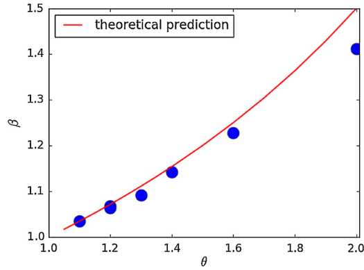
Fig. 6. Plot of the exponent \beta as a function of \theta , obtained from a power-law fit on r(t) versus t . The theoretical prediction of Eq. (9) is shown in red. See [37] for details.
