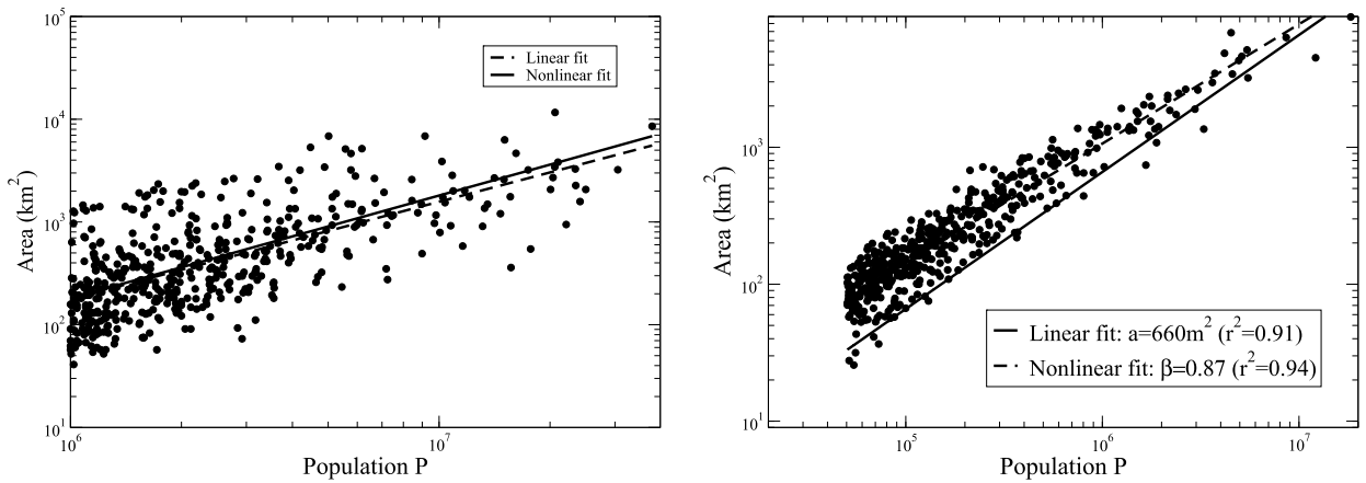
Fig. 3. Area versus population for different regions in the world. (Left) Area of the 494 world cities with population larger than 1 million inhabitant. Both the linear and nonlinear fits are acceptable and very close to each other (data from various sources compiled by Wikipedia). (Right) US Urban areas with population over 50, 000 (data from the 2010 Census population). Here also both linear and nonlinear fits are acceptable and a more thorough statistical analysis is needed (such as in [26], for example).
