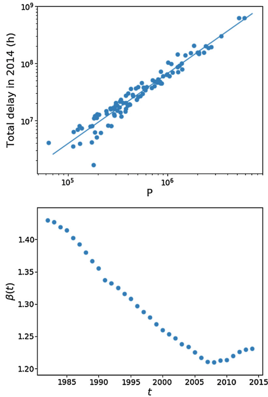
Fig. 9. (Top) Plot of the annual delay \delta\tau versus the number of drivers P for all cities in 2014. The straight line is a power-law fit in this log–log representation and gives an exponent value \beta \approx 1.23 (and R^2 = 0.93 ). (Bottom) Scaling exponent \beta(t) for the delay computed for each year separately, from 1982 to 2014. All these values are consistent with a superlinear behavior found in [57]. Figure taken from [56].
