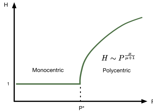
Fig. 8. Number of activity centers versus population for the model discussed in the text: we observe a monocentric-polycentric transition for a value P^* that depends on the city.
