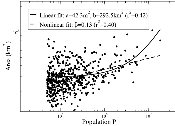
Fig. 4. Area versus population for urban areas in Japan (data from the UN, Demographic Yearbook 2012).
