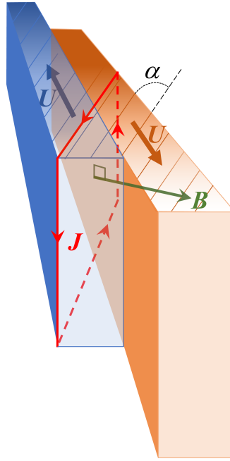
Figure 1. Illustration of the anisotropic dynamo mechanism. The two moving parts are made of the same homogeneous material. The maximum electrical conductivity is along vertical planes parallel to the lines drawn at the top surfaces. The current density loop \mathbf{J} (in red) induces a magnetic field \mathbf{B} (in green). The component of \mathbf{B} which is perpendicular to \mathbf{U} reinforces the vertical component of \mathbf{J} in each moving part, through the cross product \mathbf{U} \times \mathbf{B} (Ohm's law), making the dynamo possible (provided a velocity threshold is exceeded to compensate for Joule dissipation).
