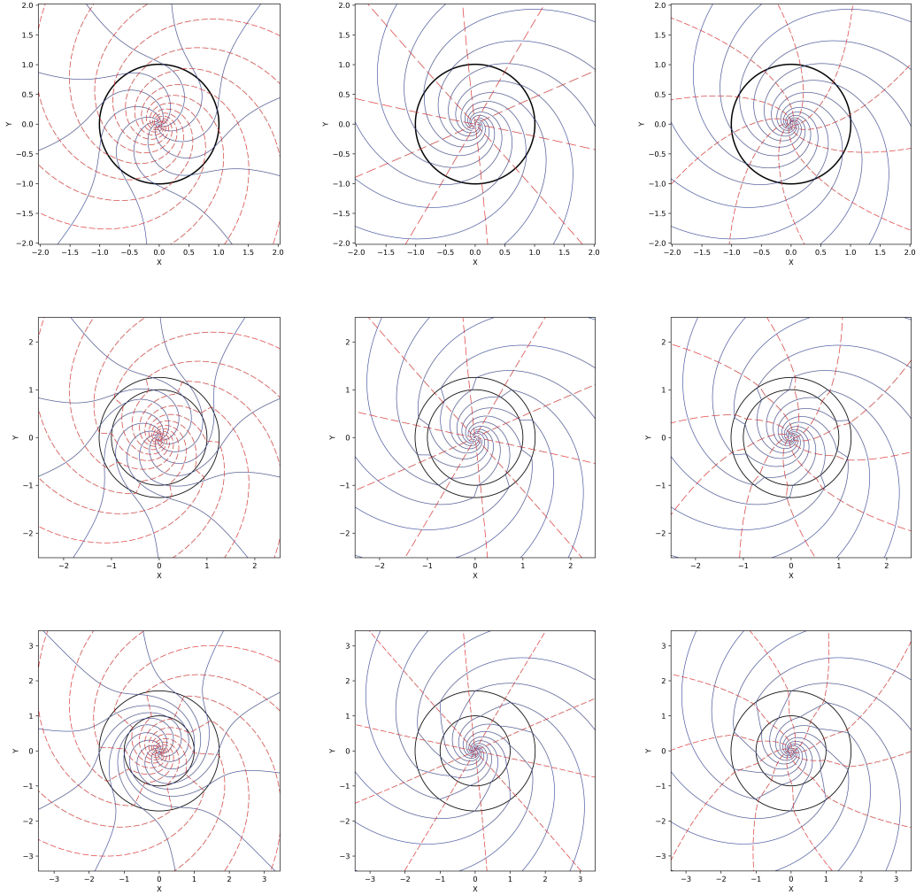
Figure 4. Plots of the magnetic field lines (full-blue) and the electric current lines (dashed-red) in the horizontal plane (x, y) , for the three cases \text{Cu}^{(\perp)}\text{Ka}^{(\parallel)} (left column), \text{Fe}^{(\perp)}\text{Sn}^{(\parallel)} (middle column), \mu\text{m}^{(\perp)}\text{Sn}^{(\parallel)} (right column), for \alpha/\pi = 0.15 , \beta = 0 , k = 1.5 and, from top to bottom, e = 1\%, 25.7\%, 71.4\% .
