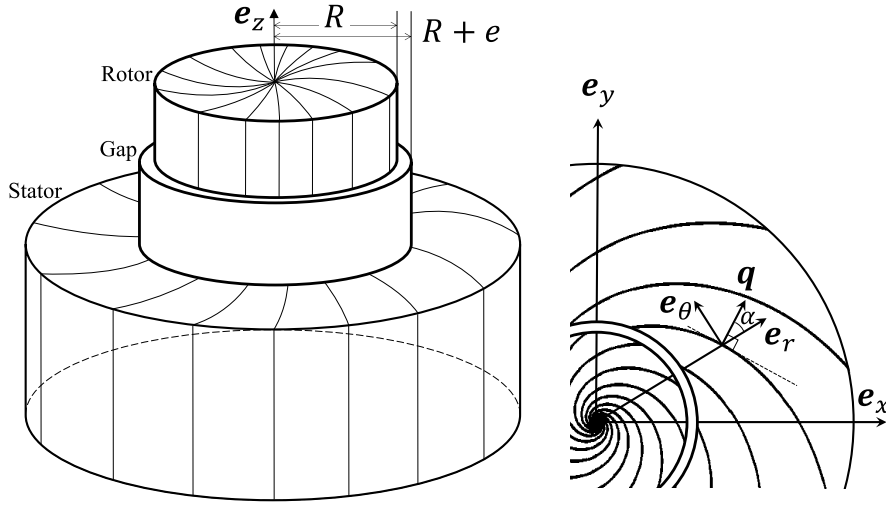
Figure 2. Left: Exploded view of the rotor surrounded by the gap, itself surrounded by the stator. Right: The logarithmic spirals in the rotor and stator correspond to the direction of the electric current (resp. magnetic field) for \sigma^\perp \gg \sigma^\parallel (resp. \mu^\perp \gg \mu^\parallel ), in the horizontal plane seen from above. They are perpendicular to \mathbf{q} .
