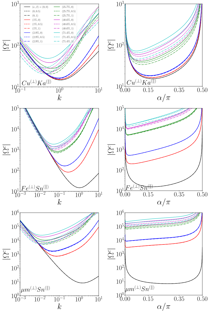
Figure 3. The dynamo threshold |\Omega^c| is plotted, either (left) versus the wave number k for a pitch angle \alpha = 0.15\pi , or (right) versus \alpha for k = 1.5 . The top row corresponds to the copper (⊥) /kapton (||) case, the middle row to the iron (⊥) /tin (||) case, the bottom row to the \mu -metal (⊥) /tin (||) case. Each curve corresponds to a couple (e, \beta) , with e \in \{0; 10^{-2}; 2.9 \times 10^{-2}; 2.57 \times 10^{-1}; 4.86 \times 10^{-1}; 7.14 \times 10^{-1}\} and \beta \in \{0; 0.5; 1\} .
