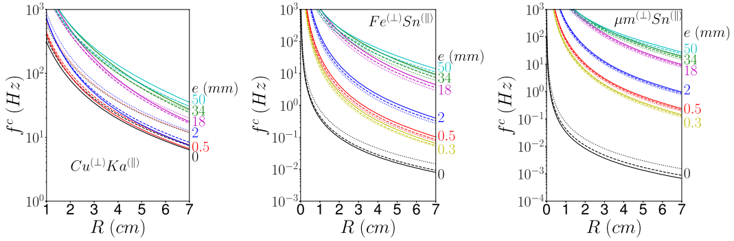
Figure 6. The critical frequency f^c (in Hz) is plotted versus the rotor's radius R \in [0, 7 \text{ cm}] for (left) the copper ^\perp /kapton ^\parallel , (middle) the iron ^\perp /tin ^\parallel and (right) the \mu -metal ^\perp /tin ^\parallel cases, with six or seven gap thicknesses e \in [0, 50 \text{ mm}] , and three values of \alpha . The solid, dashed and dotted curves correspond to \alpha/\pi = 0.15, 0.1, 0.05 . The wave number and angular velocities ratio are fixed at k = 1.5 and \beta = 0 .
