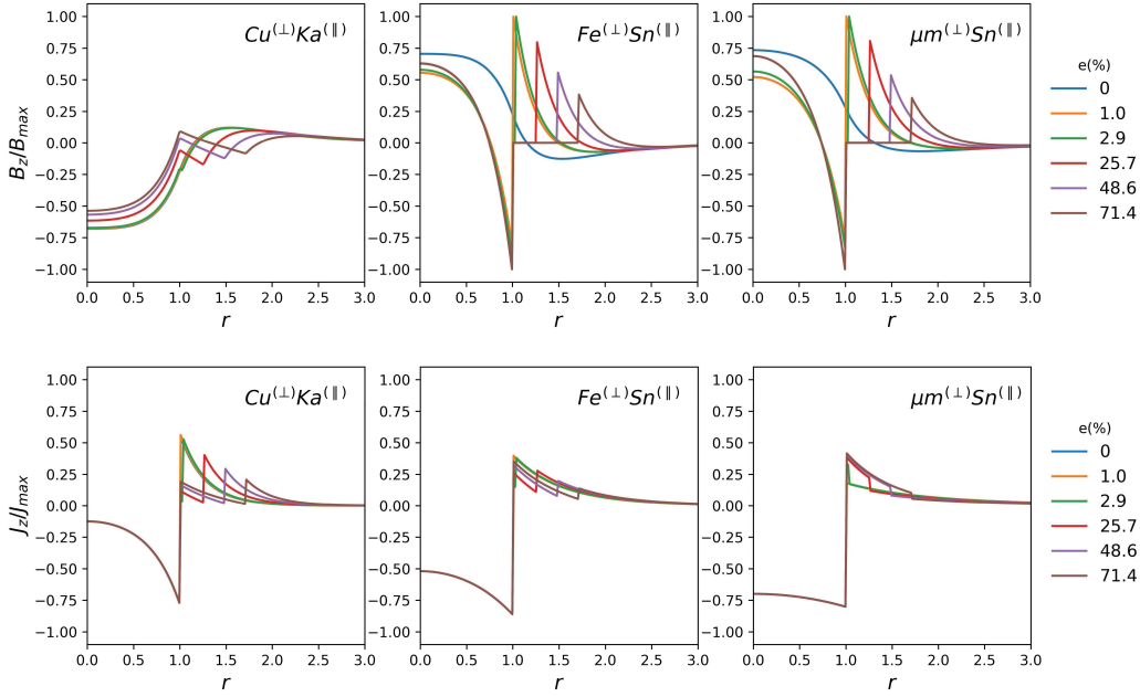
Figure 5. Plots of B_z(r)/B_{\max} (top) and J_z(r)/J_{\max} (bottom), for the three cases \text{Cu}^{(\perp)}\text{Ka}^{(\parallel)} (left column), \text{Fe}^{(\perp)}\text{Sn}^{(\parallel)} (middle column), \mu\text{m}^{(\perp)}\text{Sn}^{(\parallel)} (right column), for \alpha/\pi = 0.15 , \beta = 0 , k = 1.5 , and e = 0\%, 1\%, 2.9\%, 25.7\%, 48.6\%, 71.4\% .
