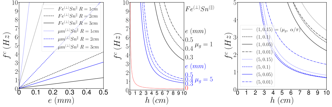
Figure 7. The critical frequency f^c (in Hz) is plotted: (left) versus the galinstan gap thickness e for the iron ⊥ /tin ∥ and the \mu -metal ⊥ /tin ∥ cases, for three values of rotor's radius R \in \{1, 2, 3\} cm, for k = 1.5 and \alpha/\pi = 0.15 ; (middle) versus the magnetic vertical wavelength h for the iron ⊥ /tin ∥ case, for four values of gap's thickness e \in \{0, 0.3, 0.4, 0.5\} mm, for R = 1.5 cm and \alpha/\pi = 0.15 ; (right) versus the magnetic vertical wavelength h for the iron ⊥ /tin ∥ case, for four values of \alpha/\pi \in \{0.01, 0.05, 0.1, 0.15\} , for R = 1.5 cm and e = 0.3 mm. In all cases, \beta = 0 . In the middle and right subfigures two values of \mu_g are considered \mu_g \in \{4\pi \times 10^{-7}, 20\pi \times 10^{-7}\} .
